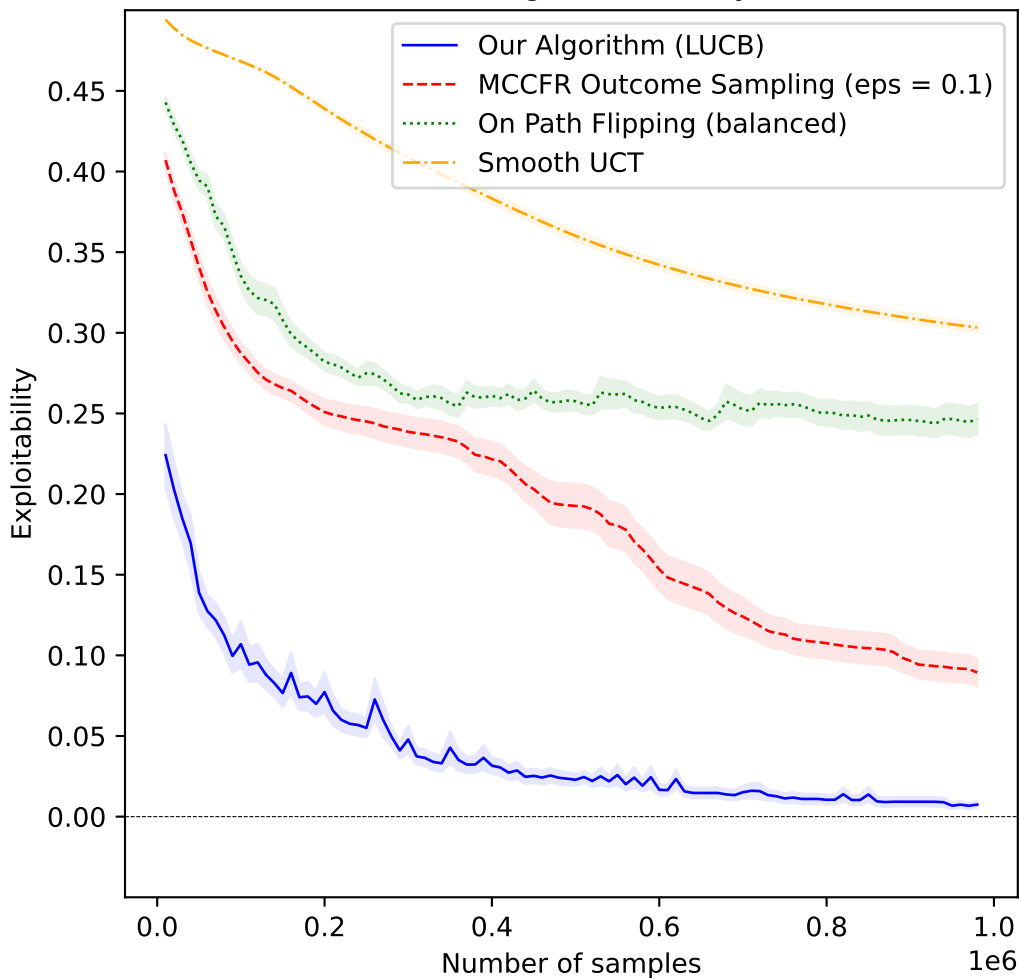
RBT, Best Algorithms, Player o
